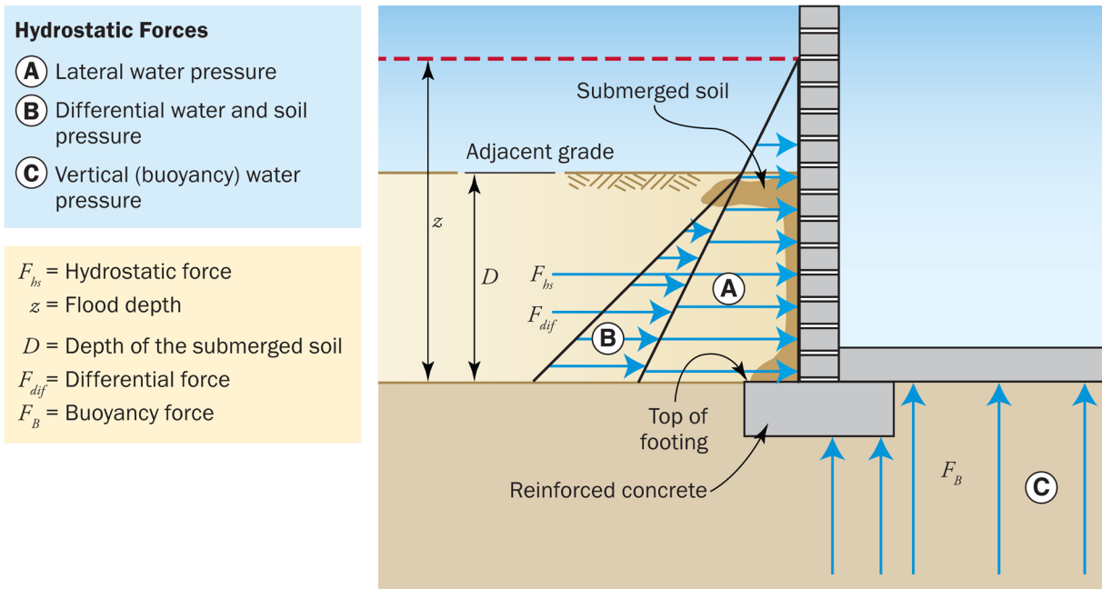
Figure 6. Combination soil/water hydrostatic and buoyancy forces for submerged soils
