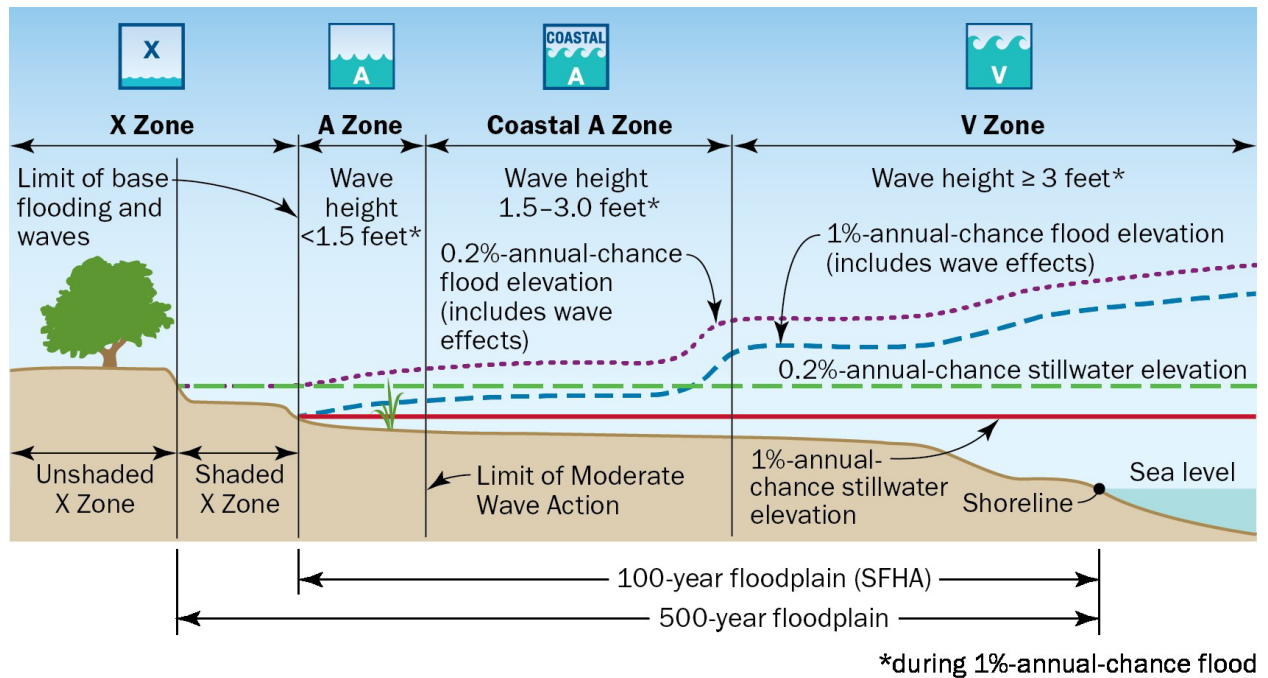
Figure 1. Typical flood zones from coastal flood sources
