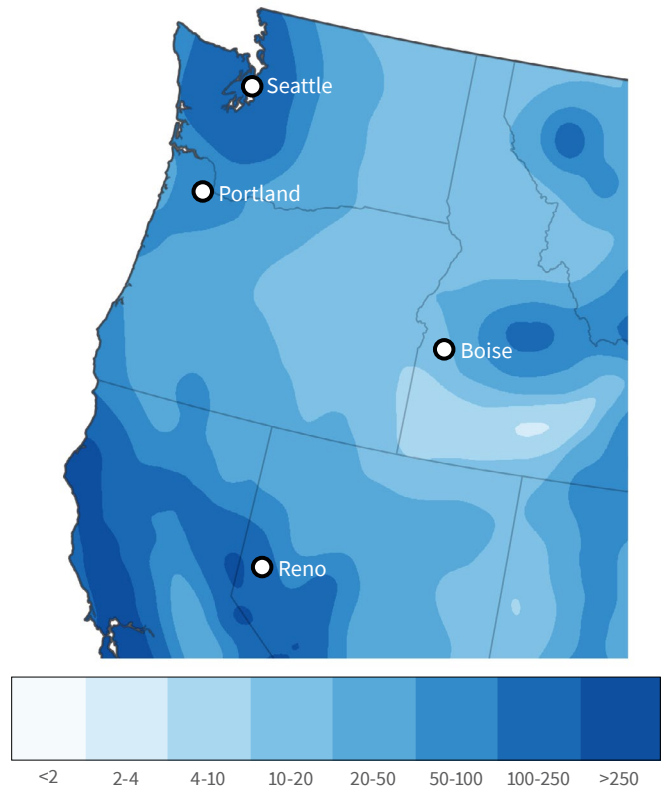
Expected number of occurrences of damaging earthquake shaking in 10,000 years.
